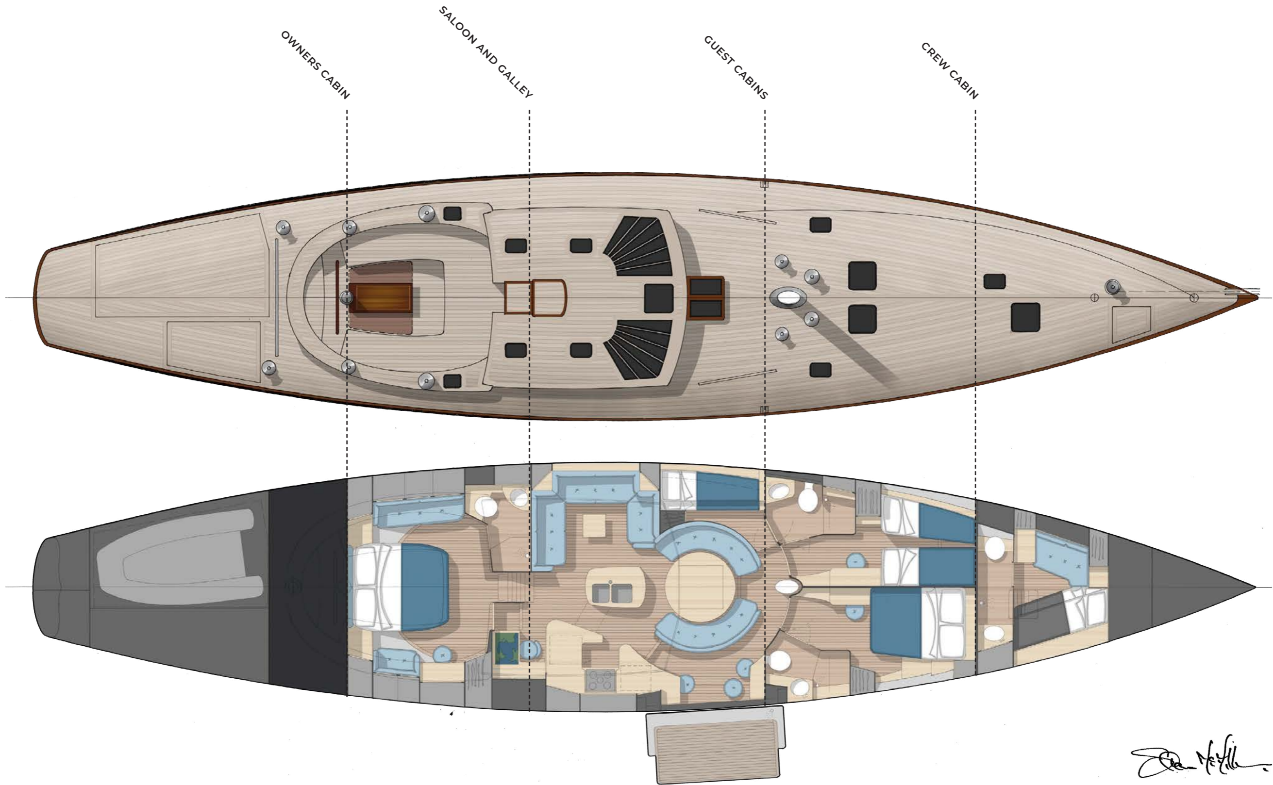
SPIRIT 84 GENERAL ARRANGEMENT PLAN
